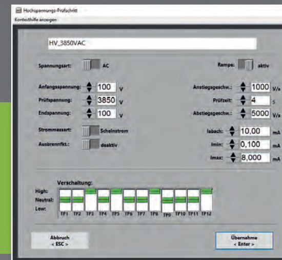
High-voltage test plan with switching matrix
